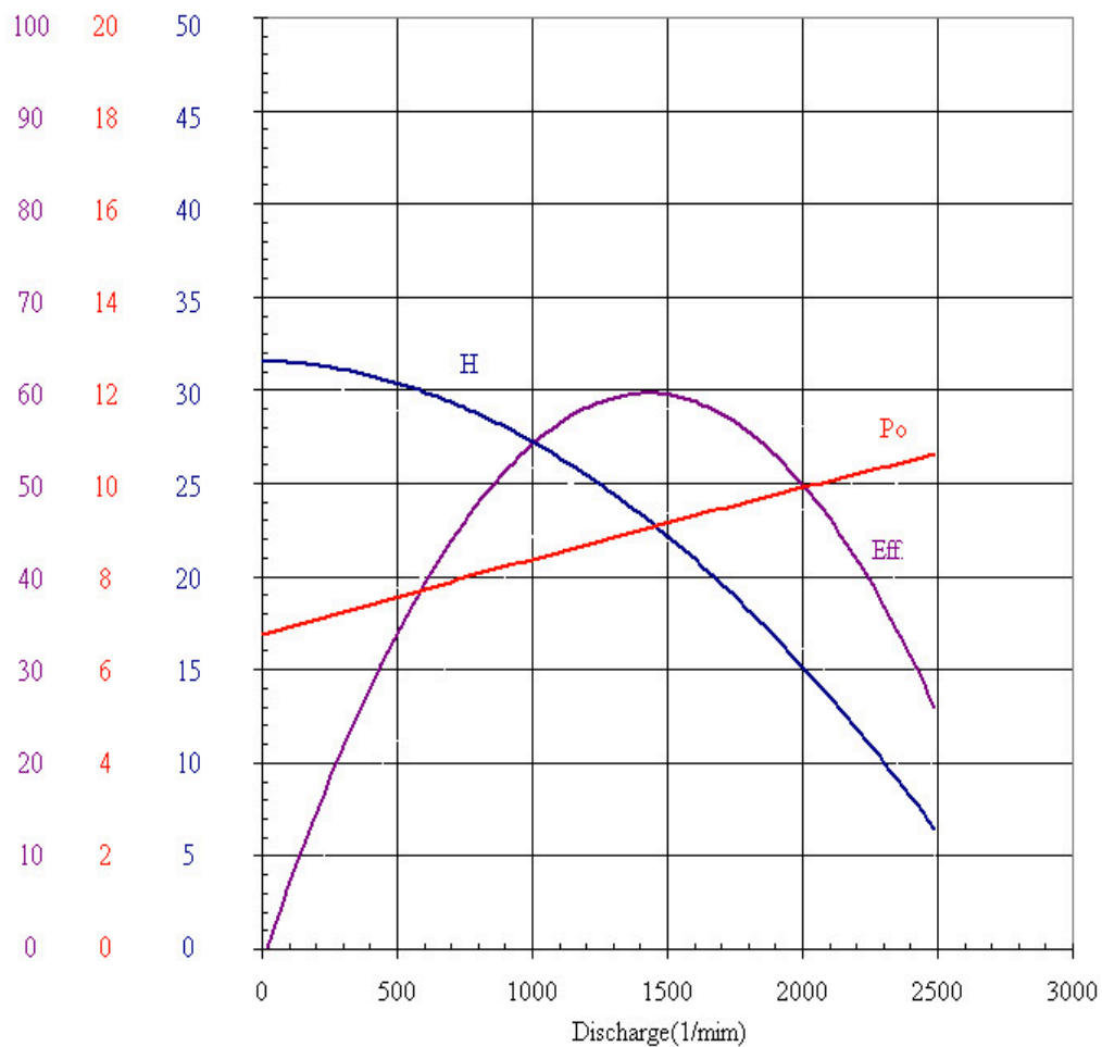
PUMP Performance Curve
